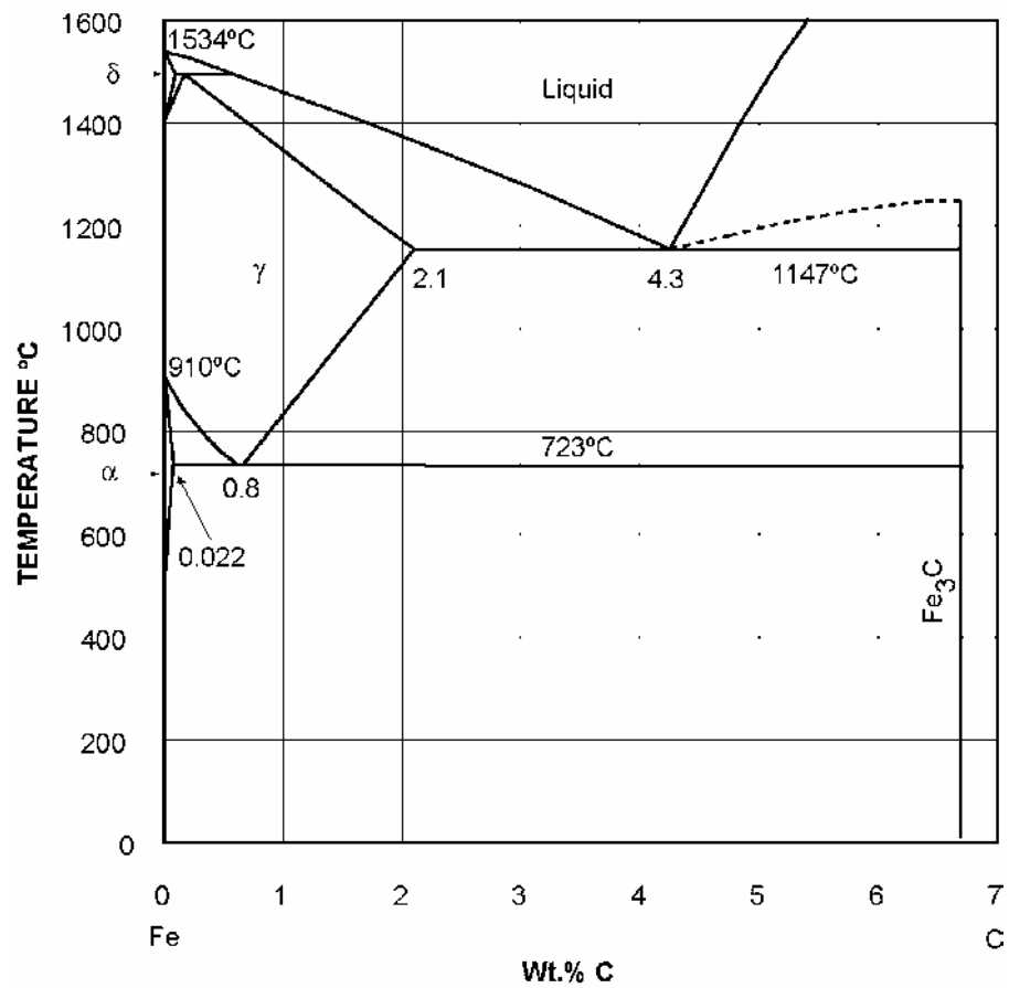
Figure 6.3 Iron – Carbon equilibrium diagram
